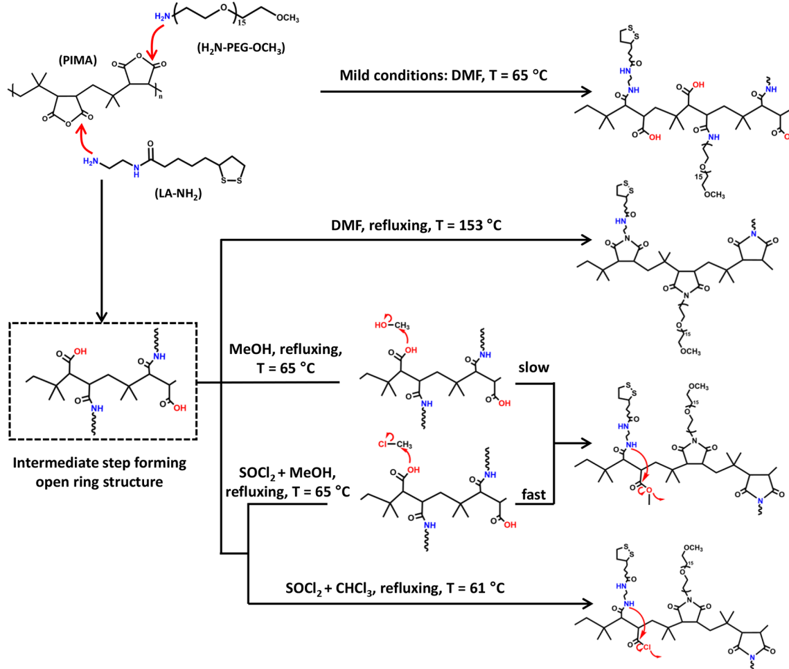
Figure 4. Summary of the proposed transformation accompanying the addition reaction when carried out: under mild conditions yielding ring open structure (top) and under refluxing conditions in DMF, methanol, or in the presence of added \text{SOCl}_2 (bottom); the latter conditions yield closed ring structures. Note that formation of the cyclic imide rings, under the various conditions, is still preceded by a ring opening step.
