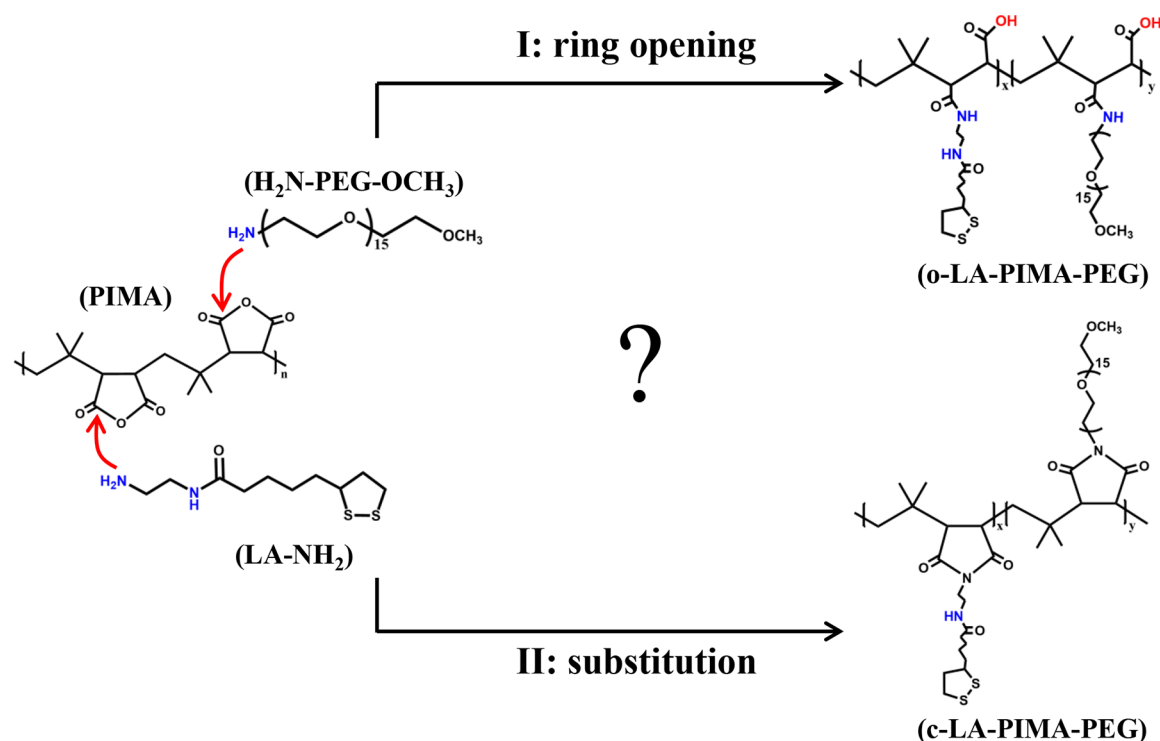
Figure 1. Schematic representation showing the addition reaction between poly(isobutylene- alt -maleic anhydride) and \text{H}_2\text{N}-\text{R} motifs ( \text{R} = \text{PEG}-\text{OMe} or/and LA). The two proposed pathways describing (I) anhydride ring opening coupled with amide-bond formation with \text{R} , or (II) substitution reaction yielding cyclic imide-bound \text{R} .
